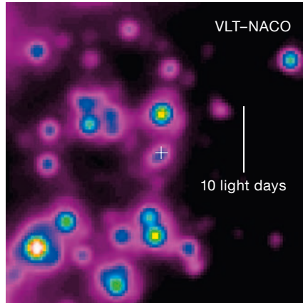
Figure 2. The innermost arcsecond of the Galactic Centre. Left: NACO image at the VLT diffraction limit, showing S-stars and the location of the black hole Sgr A* (cross). Right: A simulated image with MICADO, extrapolating from the measured luminosity function and density profile. Proper motions of hundreds of stars will be measurable, providing detailed constraints on the black hole mass and extended mass distribution.
